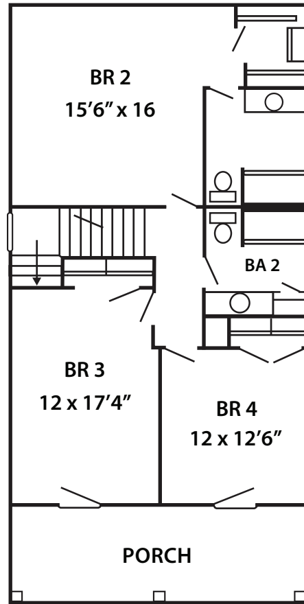
SECOND FLOOR 960 sq. ft.
