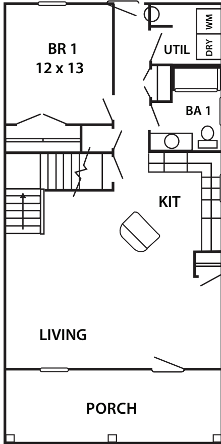
FIRST FLOOR 960 sq. ft.
